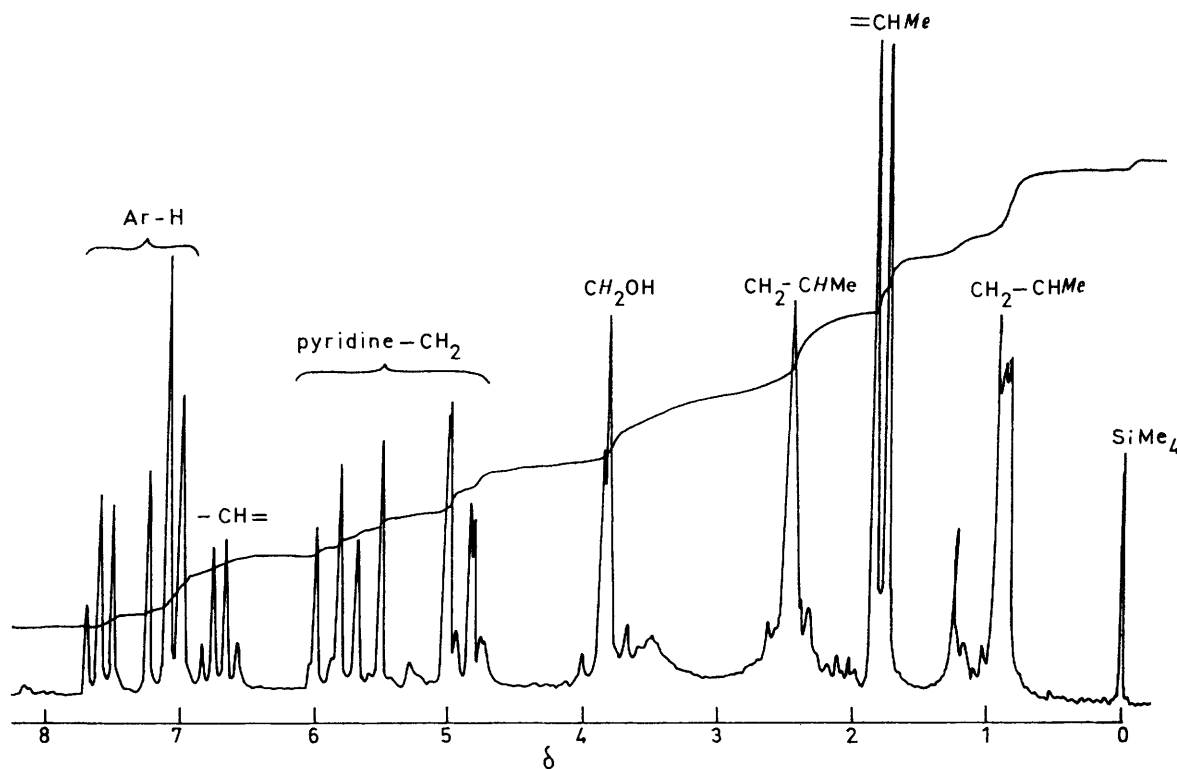
1 H N.m.r. spectrum of pyridine-retronecate (5) at 80 MHz
